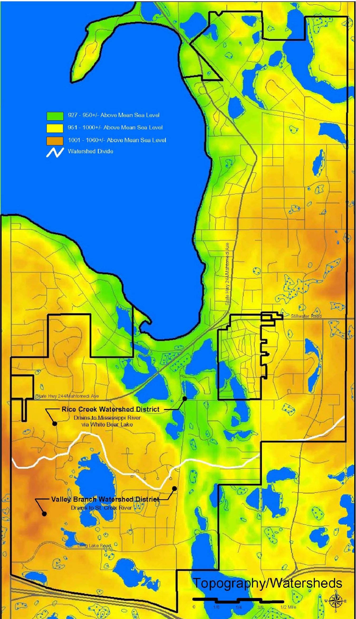
Figure 5-1: Topography Watersheds
